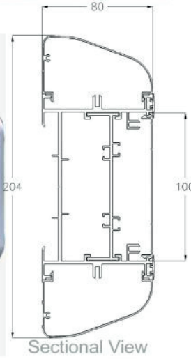
Sectional View
